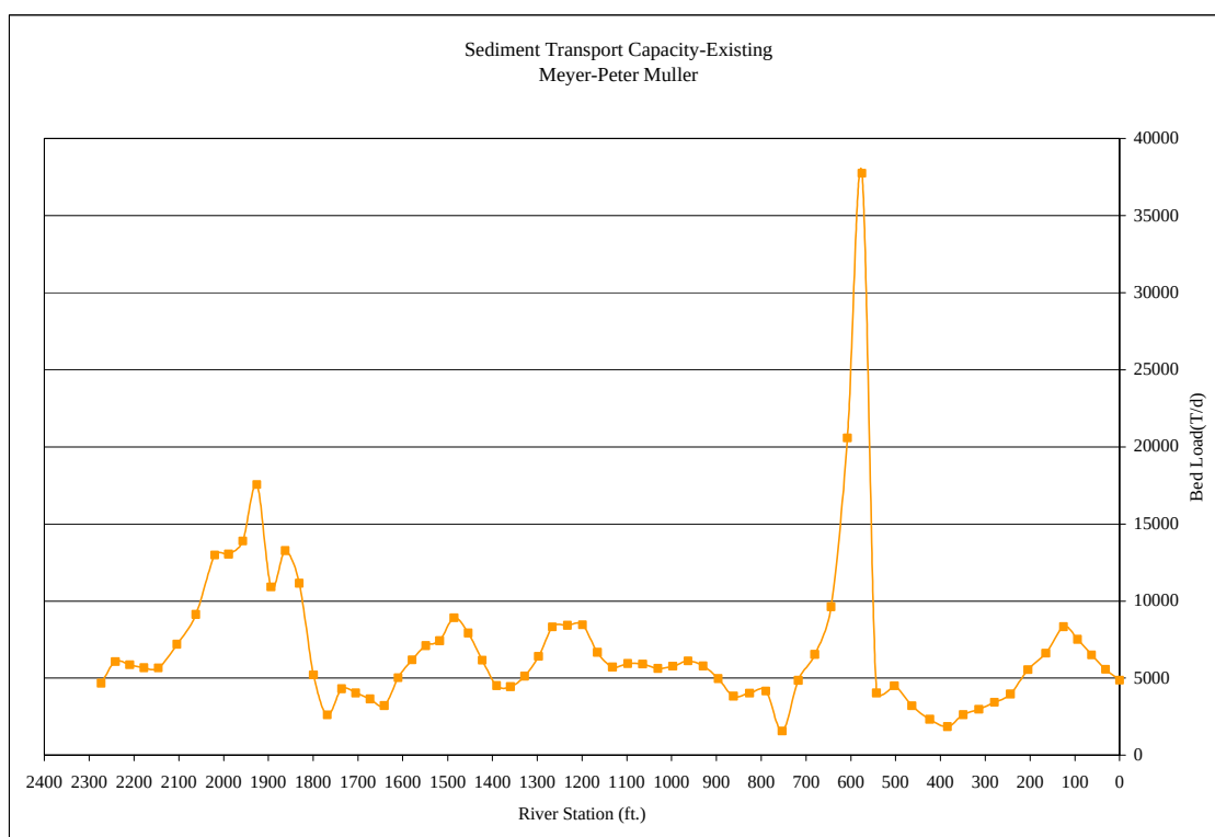
Figure 9. Bedload transport capacity using Meyer-Peter Muller equation through the project rea
