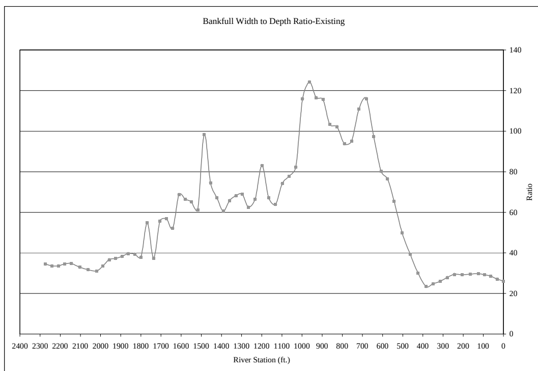
Figure 4. Bankfull channel width to depth ratio through the project reach.
